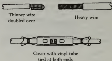
FIGURE 4-110. Reducing wire size with a permanent splice.
